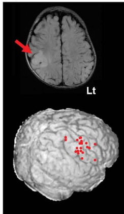
(A) MRI ; MEG-ECD (B) EEG: 1y/o (pre-operation)
