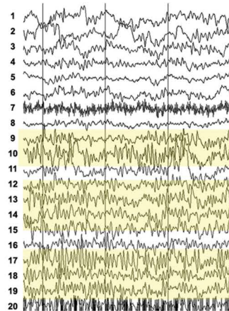
(C) ECoG: (pre-resection)
