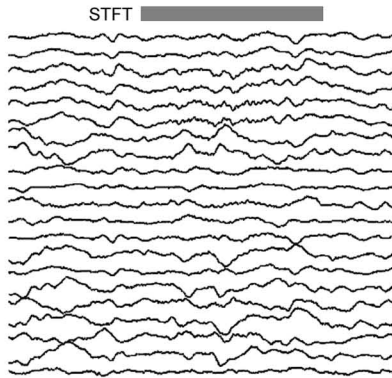
(A) MRI ; MEG-ECD (B) EEG: 1y/o (pre-operation)
