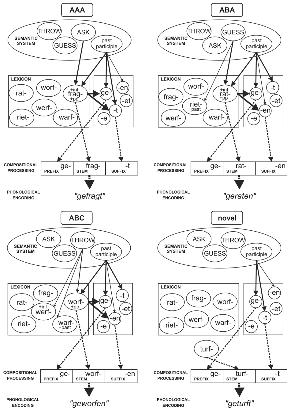
Figure 4. Schematic depiction of the mechanisms that SAM proposes for the production of German past participle forms. AAA past participles (e.g., ge fragt [asked]); ABA past participles (e.g., ge raten [guessed]); ABC past participles (e.g., ge worfen [thrown]); past participle of a novel verb (e.g., ge turft; suffix –t is expected). Lexical representations and affixes are activated by semantic and grammatical processes (the latter are not shown). Verb stems and suffixes are stored separately. Solid arrows indicate activation; line thickness corresponds to degree of activation; dashed arrows indicate that a given representation has been selected.
