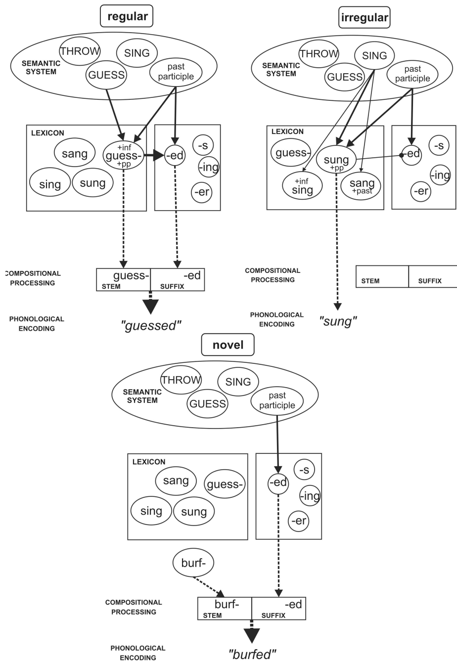
Figure 3. Schematic depiction of the mechanisms that SAM proposes for the production of English past tense and past participle forms. Regular inflections ( guessed ); irregular inflections ( sung ); and novel verbs ( burfed ). Verb stems are encoded in the lexicon, separately from suffixes. Lexical representations and affixes are activated by semantic and grammatical processes (the latter are not shown). Solid arrows indicate activation, with line thickness indicating degree of activation; dashed arrows indicate that a given representation has been selected; the line with a black, round endpoint indicates inhibition. The suffix -ed is always
