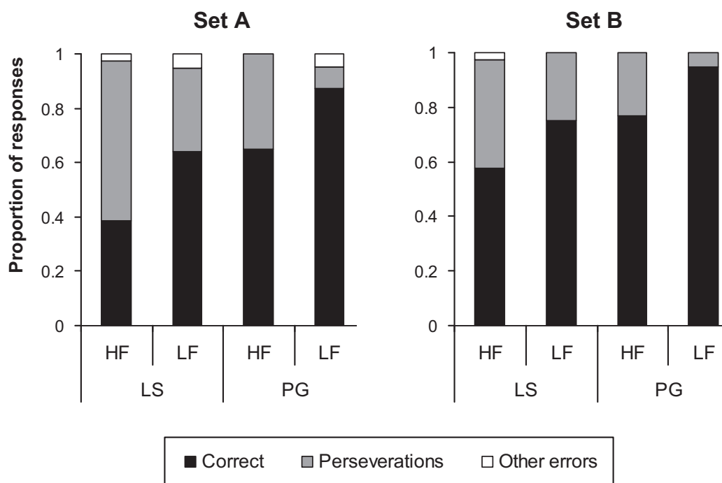
Fig. 1. Correct responses, perseverations and other errors. HF, high frequency trial; LF, low frequency trial.
