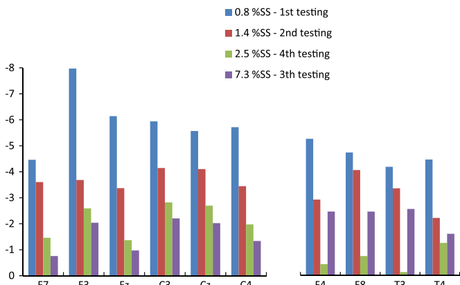
Fig. 5. Mean CNV amplitude ( \mu\text{V} ) of the response locked analysis at all test sessions. Bars are colored corresponding to % SS during conversation.
