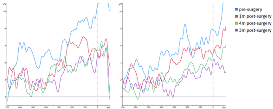
Fig. 7. The late CNV at Cz for all test sessions, the 700 ms preceding the averaging point are shown. On the left, the stimulus locked analysis is displayed in which 0 ms represents S2 onset. On the right, response locked analysis is depicted in which 0 ms represents EMG onset. Negative is plotted upwards.
