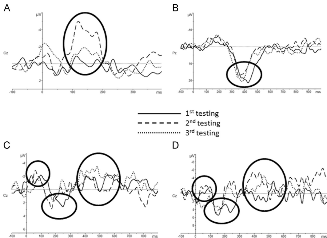
Fig. 8. Event-related potentials (ERP) evoked by the phonological tasks. Latency ( x -axis) is represented in milliseconds (ms) and amplitude ( y -axis) in microvolts ( \mu\text{V} ). Negative is plotted upwards. Top: the unattended and attended phoneme discrimination tasks: (A) MMN at Cz (B) P300 at Pz. Bottom: the word recognition tasks evoked the successive peaks N100, P200 and N400: (C) real words at Cz (D) pseudowords at Cz.
