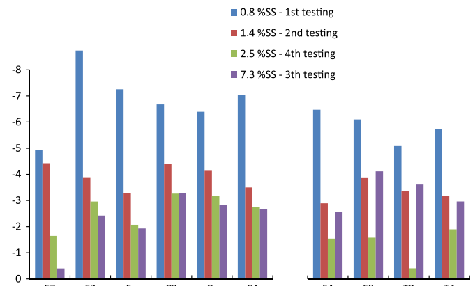
Fig. 6. Mean CNV amplitude ( \mu\text{V} ) of the stimulus locked analysis at all test sessions. Bars are colored corresponding to % SS during conversation.
