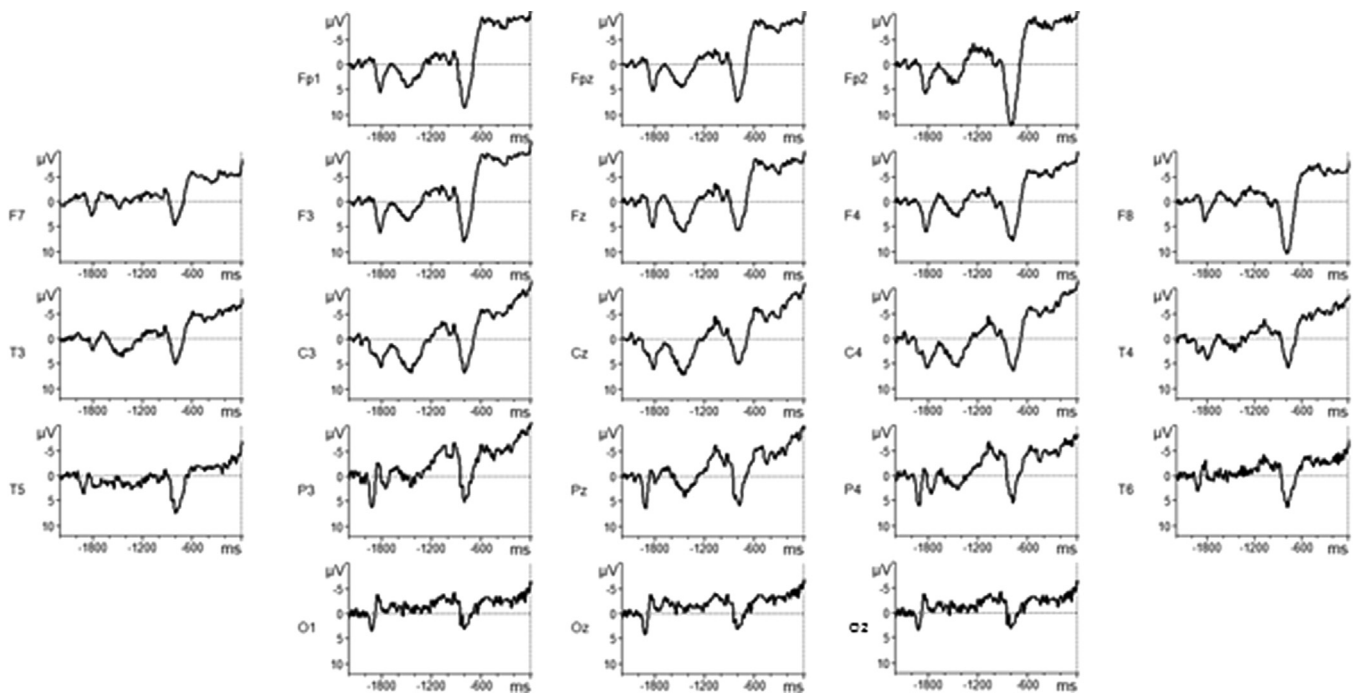
Fig. 4. Stimulus locked analysis of all electrodes at the first test session. Latency ( x -axis) is represented in milliseconds (ms) and amplitude ( y -axis) in microvolts ( \mu\text{V} ). Negative is plotted upwards. Baseline is the first 200 ms of the epoch i.e. 200 ms before S1 onset. The 0 ms point is S2 onset.
