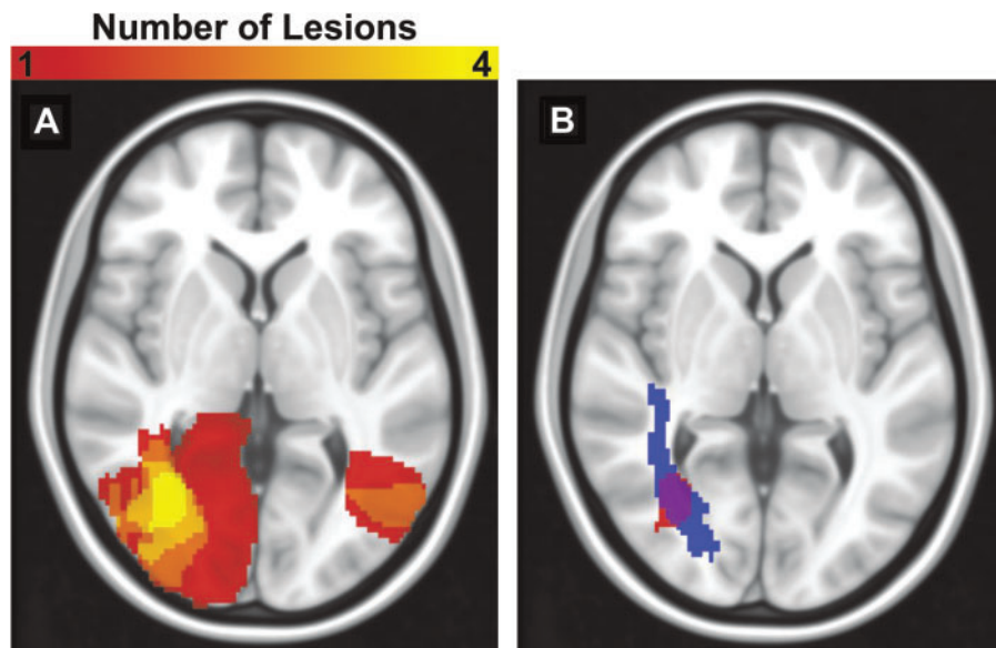
Fig. 3. Normalized lesions were overlapped from all four cases of lesional visual hypoemotionality. (A) Lighter shades of orange represent greater degree of overlap. All four lesions overlap in the posterior white matter of the right hemisphere. (B) The maximum overlap (red) fell over the right inferior longitudinal fasciculus (in blue).
