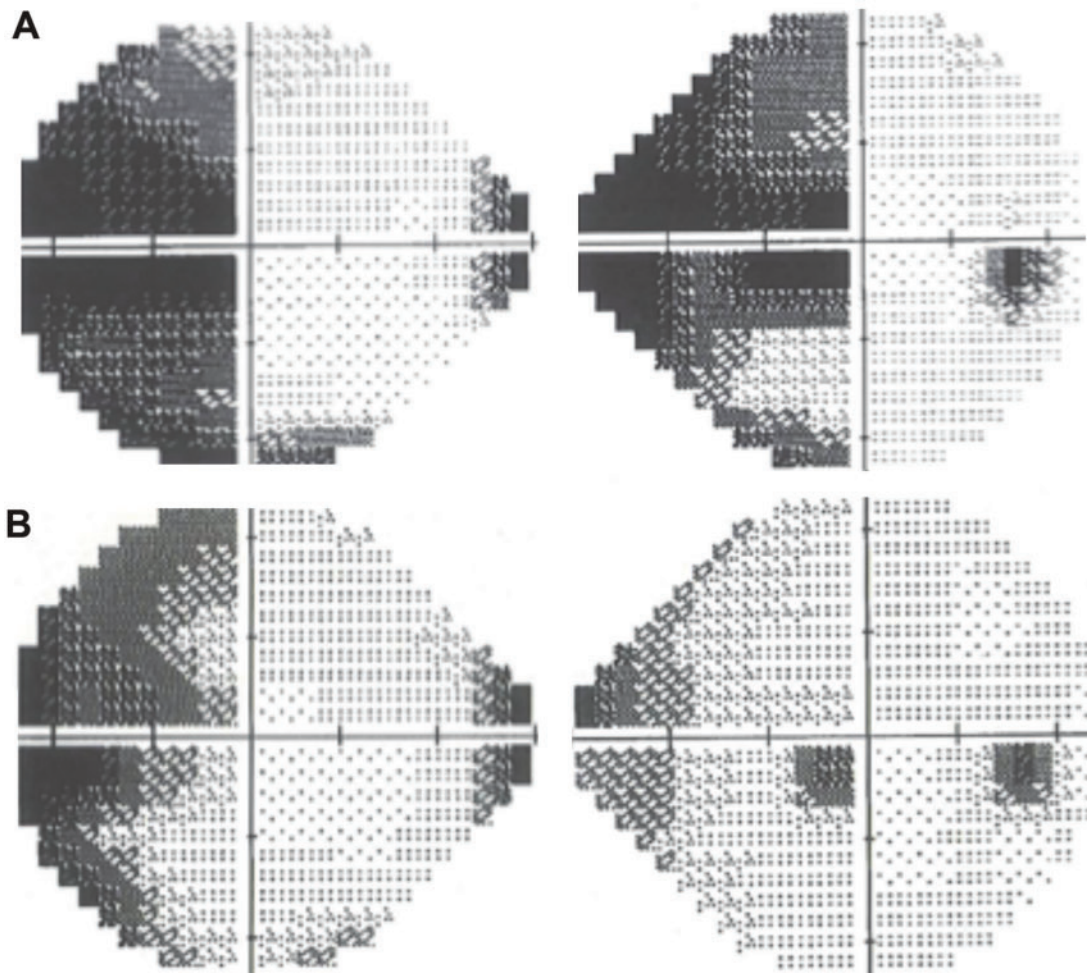
Fig. 1. Visual field analyses of left visual field deficit. Analyses conducted 1 month (A) and 11 months (B) following the intraparenchymal hemorrhage demonstrate improvement in visual deficit.
