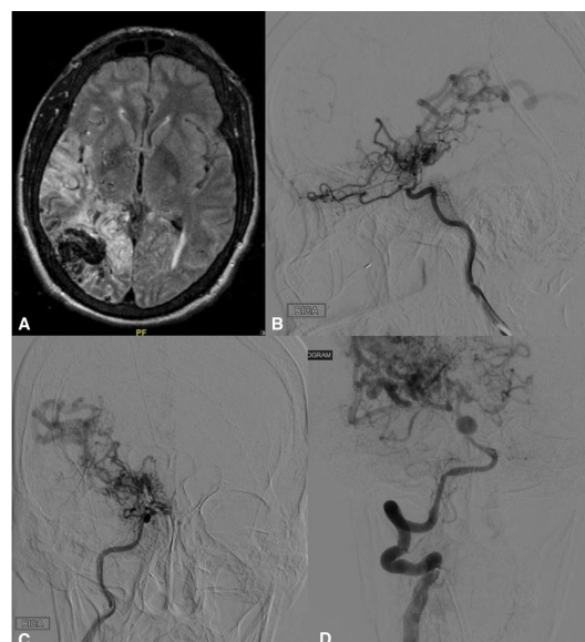
Figure 2 MRI brain fluid-attenuated inversion recovery (FLAIR) sequence (A) shows right parietal hyperintensity from venous hypertension-induced oedema and large arteriovenous malformation. Four vessel angiogram shows right terminal internal carotid artery occlusion and moyamoya disease distally (B and C) and basilar artery aneurysm (D).
