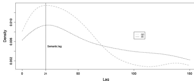
Figure 5. The probability density of lexical perseveration by lag for QD and XR. The vertical line (lag 21) represents the average lag between two semantically-related items, calculated as the distance between each item and the next item from the same semantic category, averaged over all items. This lag coincides with the peak in the probability of producing a lexical perseveration in both participants.
