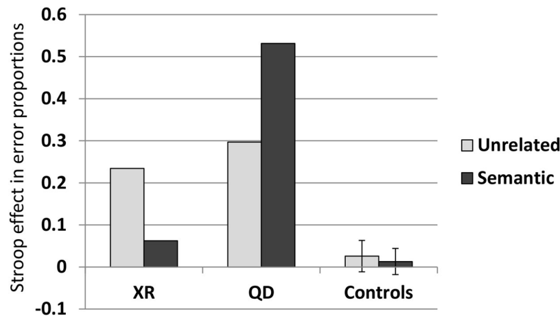
Figure 4. Stroop effects in errors (errors in reversed naming – errors in straight naming) for XR, QD, and controls ( \pm SD ) in the unrelated and semantically-related conditions in the word-Stoop task.
