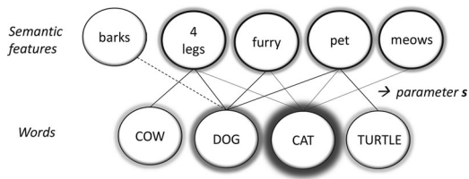
Figure 1. A schematic of the mapping of semantic features to lexical representations (words) for the target CAT. Darker circles represent higher activation, which is proportional to the number of features which send activation to the lexical representation. The dotted line represents an inactive connection.
