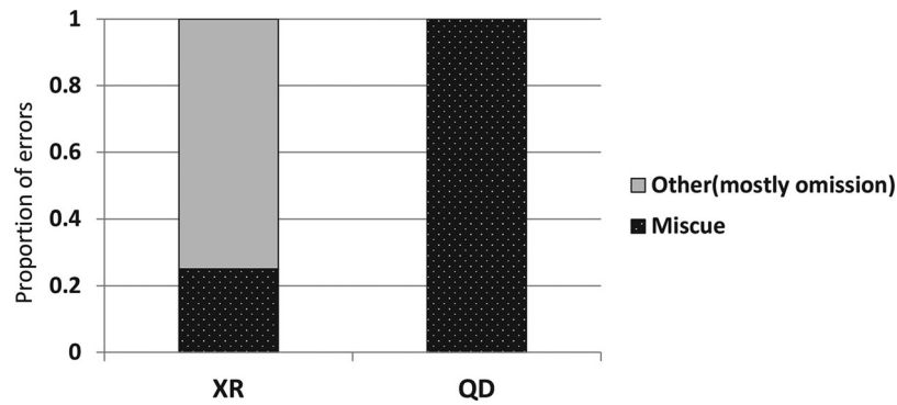
Figure 3. Proportion of miscue errors vs. other error types in all error trials in the miscue condition in XR and QD. The total number of errors in this condition is 8 for XR and 13 for QD.
