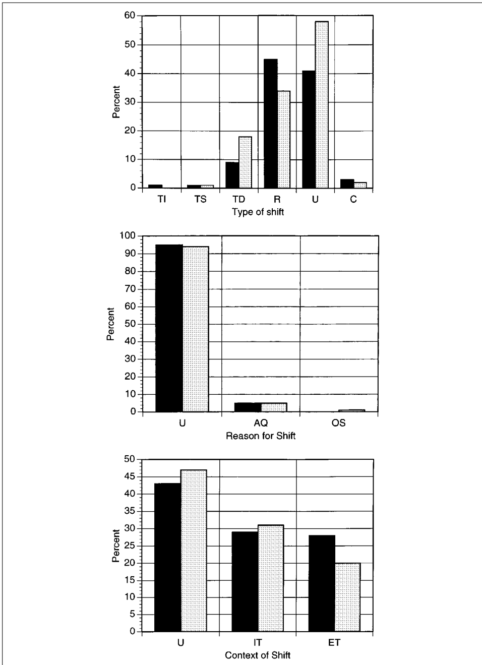
Fig. 3 – Distribution of topic shift characteristics. Black columns represent the first interview, and gray columns represent the second. a) Type of shift. TI - topic initiation, TS - topic shading, TD - topic drift, R - renewal of topic, U - unexpected, C - conflation. See Table II for operational definitions. b) Reasons for shift. U - unknown, AQ - answering previous question, OS - reacting to an outside stimulus. See Table II for operational definitions. c) Context of shift. U - unknown, IT - topic previously initiated by the patient, ET - topic previously initiated by examiner. See Table II for operational definitions.
